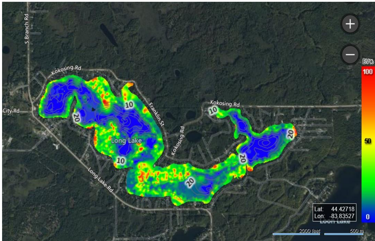
Figure 1. 2023 Aquatic vegetation biovolume map of Long Lake. Note: Blue denotes no vegetation; Green denotes low-growing vegetation; Red denotes high-growing vegetation.
