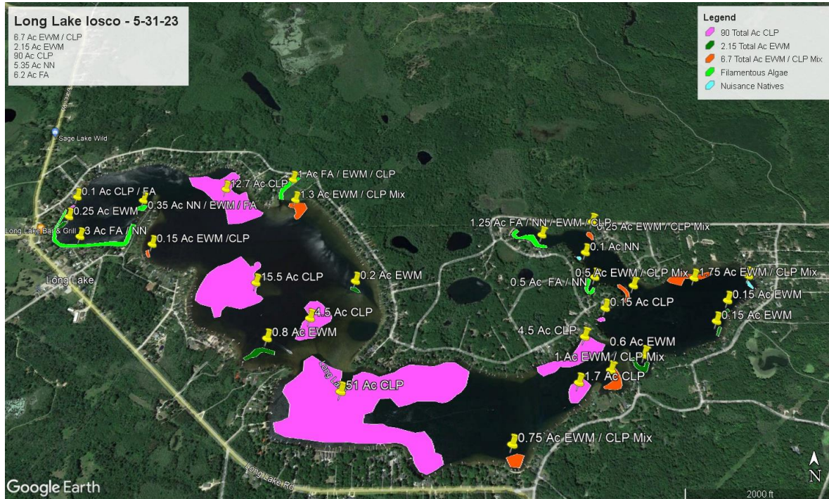
Figure 4a. Treatment map of EWM / CLP in Long Lake (May 31, 2023).
